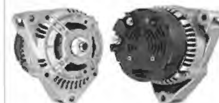
Bosch Type, 12V/90A USED ON: MERCEDES 1993-96 CARGO#: 112529 HC-Parts: CA1044IR LESTER: 13613 OEM#: 0-123-335-002, Other: ABO0034 WOODAUTO: ALT2031 WAI#: 1-1950-42BO
