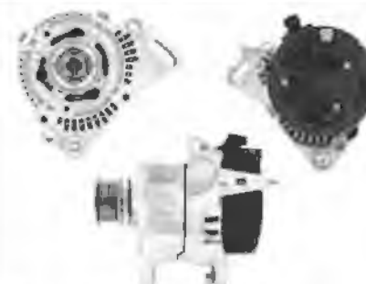
Bosch Type, 12V/90A USED ON: VOLKSWAGEN BEETLE 2.0L 1998 CARGO#: 111479 HC-Parts: CA740IR LESTER: 13605 OEM#: 0-123-320-002, 0-123-320-00 6, 0-123-340-002 Other: ABO0037 WOODAUTO: ALT10178 WAI#: 1-1808-01BO
